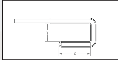
End-Tension Square Hook
